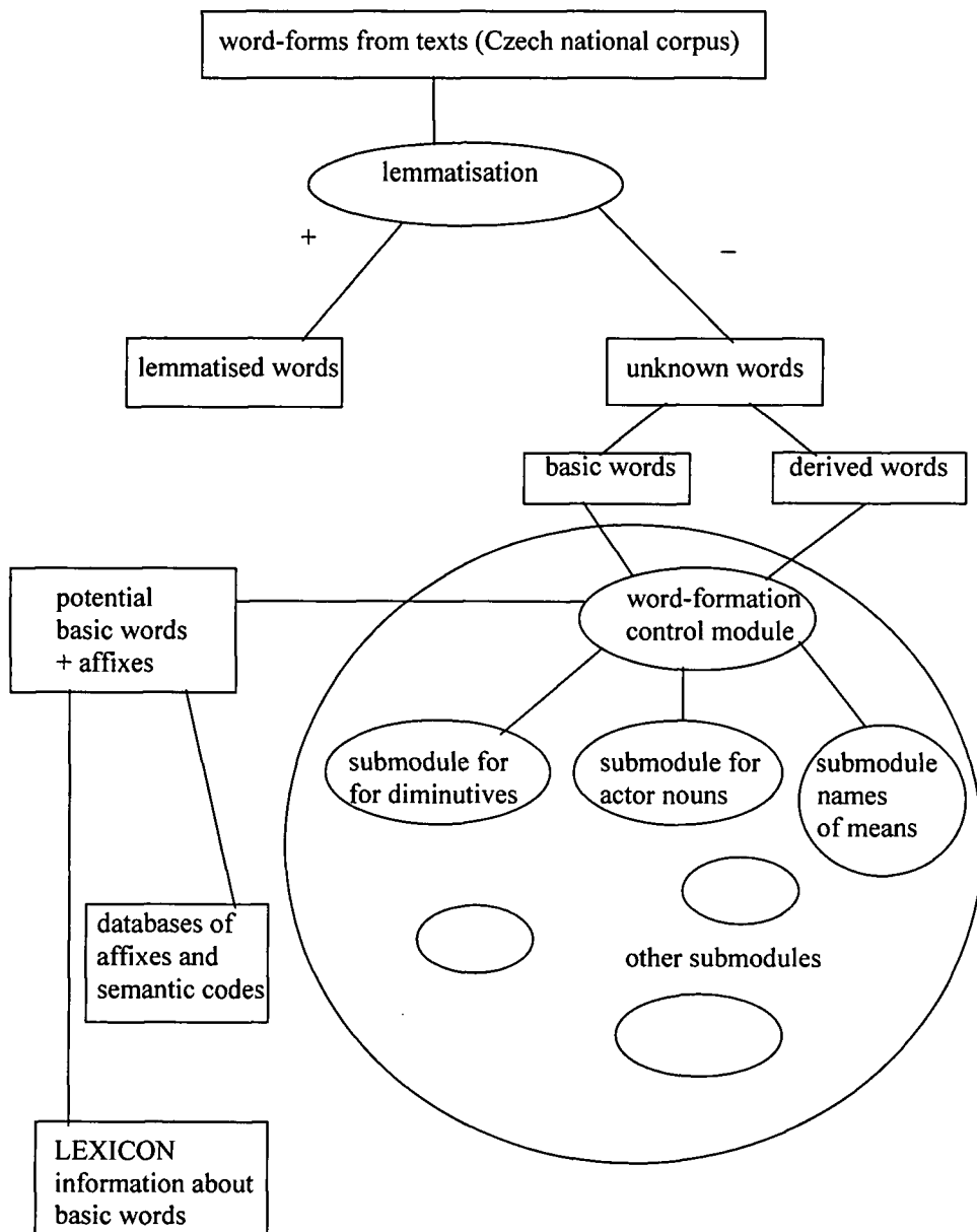
Figure 1: Processing of words from texts
